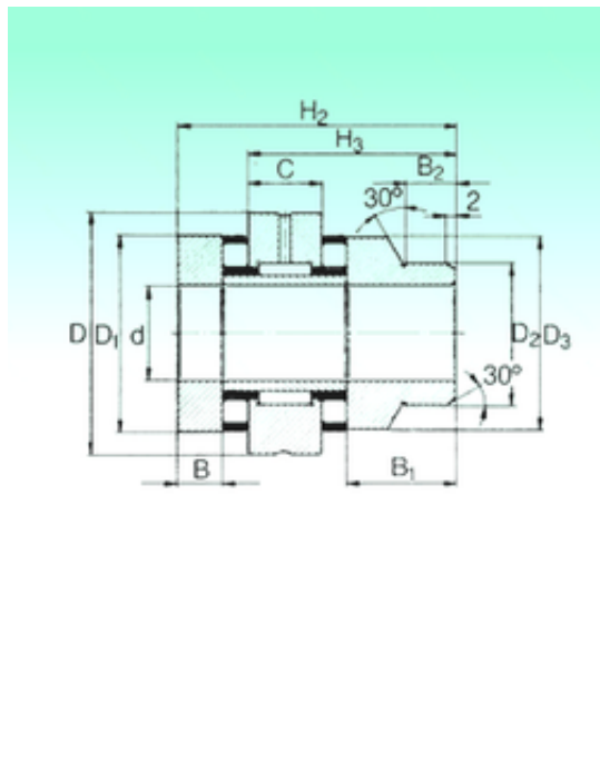
ZARN 75155 L TN Bearing 2D drawings and 3D CAD models
