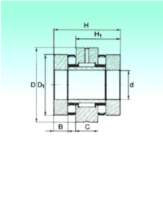
ZARN 1747 TN Bearing 2D drawings and 3D CAD models
