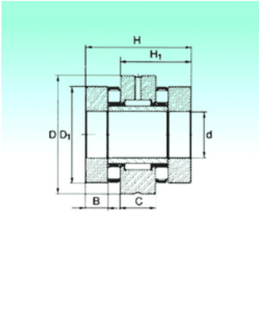
ZARN 4090 TN Bearing 2D drawings and 3D CAD models
