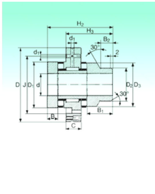
ZARF 45105 L TN Bearing 2D drawings and 3D CAD models
